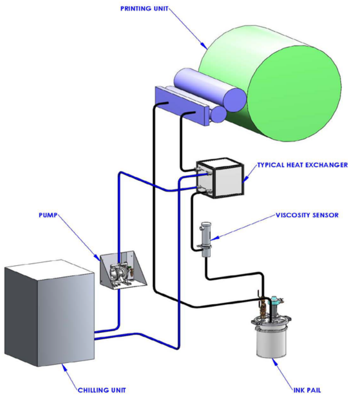
NOTE: - INSTALLATION OF A TYPICAL HEAT EXCHANGER ON THE INK FEED LINE
