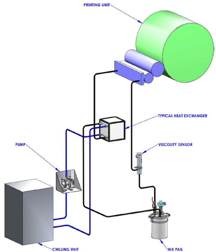
NOTE: -INSTALLATION OF A TYPICAL HEAT EXCHANGER ON THE INK RETURN LINE
